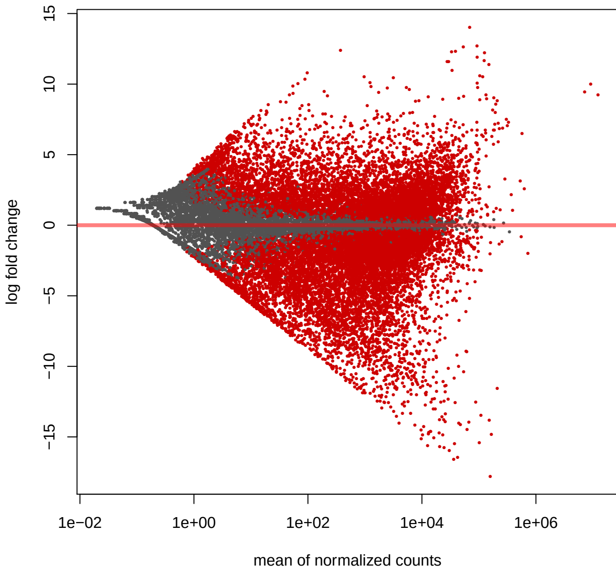
MA-plot for FactorName: Tumor vs Normal
