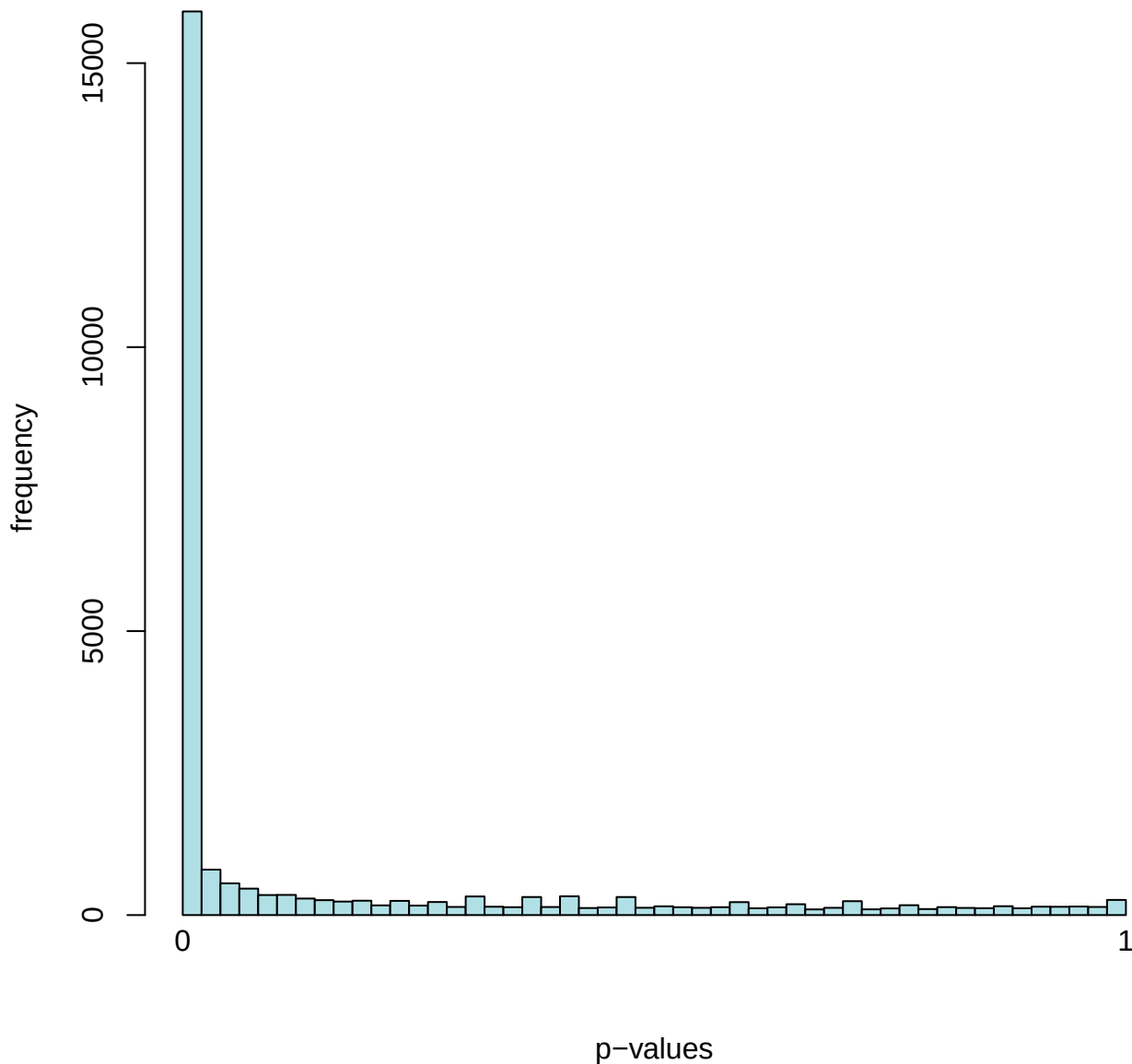
Histogram of p-values for FactorName: Tumor vs Normal
